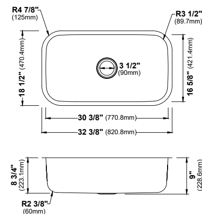
MODEL: PRU36 Stainless Steel Undermount Large Single Bowl Kitchen Sink
