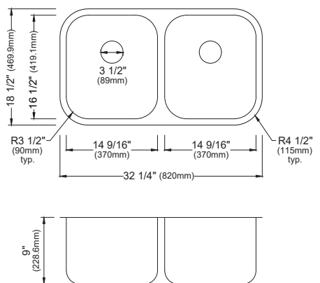
MODEL: PU51 Stainless Steel Undermount Double Bowl Kitchen Sink
