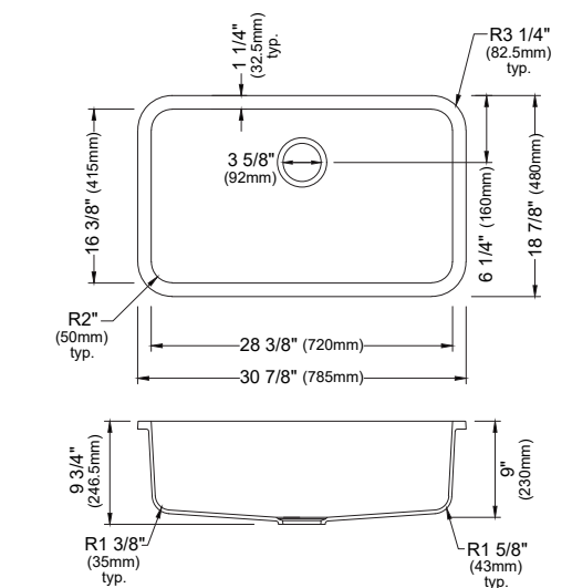
Quartz Seamless Undermount Large Single Bowl Kitchen Sink
