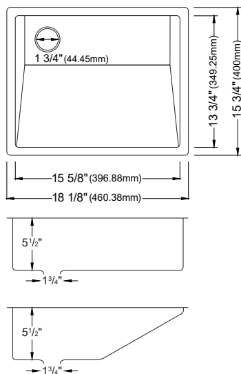
MODEL: E-505D Stainless Steel Single Bowl Seamless Undermount Vanity Sink
