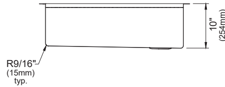
MODEL: WST-26-PK1 Stainless Steel Top Mount Large Single Bowl Kitchen Sink
