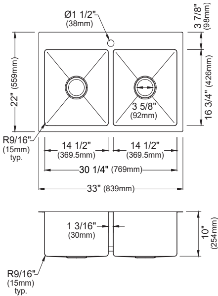
MODEL: EL-35-PK1 Stainless Steel Top Mount Double Bowl Kitchen Sink
