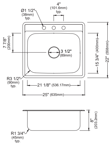
MODEL: PT30 Stainless Steel Top Mount Single Bowl Kitchen Sink
