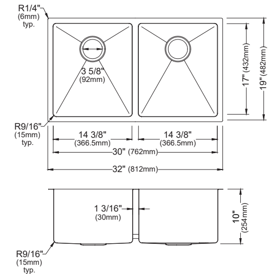
MODEL: EL-76-PK1 Stainless Steel Undermount Double Bowl Kitchen Sink
