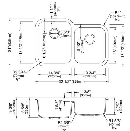
Quartz Seamless Undermount Large/Small Bowl Kitchen Sink
