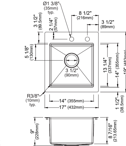
MODEL: HST1719SB Matrix Steel Top Mount Single Bowl Workstation Bar Sink
