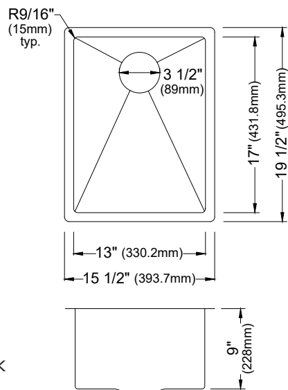
MODEL: E-510 Stainless Steel Single Bowl Seamless Undermount Bar Sink
