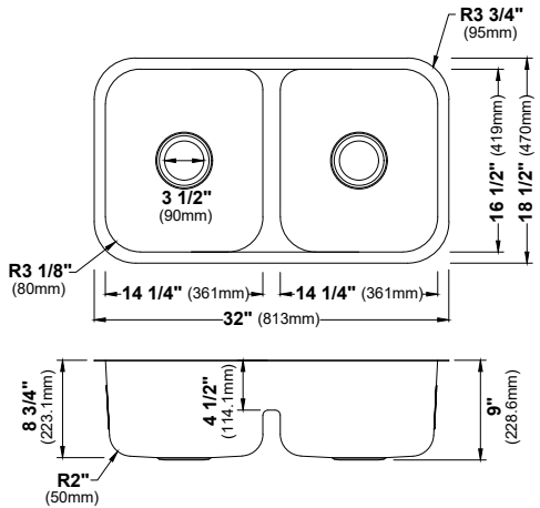
MODEL: PRU32 Stainless Steel Undermount Double Bowl Kitchen Sink
