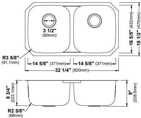
MODEL: PRU31 Stainless Steel Undermount Double Bowl Kitchen Sink
